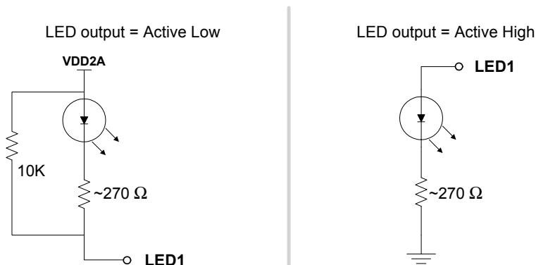
Figure 3.7 LED1 Polarity Configuration
