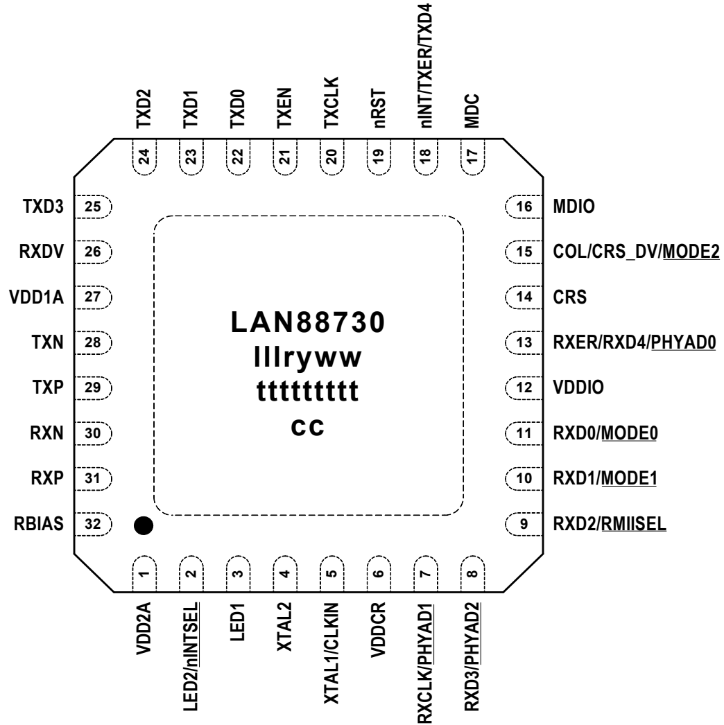
Figure 2.1 32-QFN Pin Assignments (TOP VIEW)
