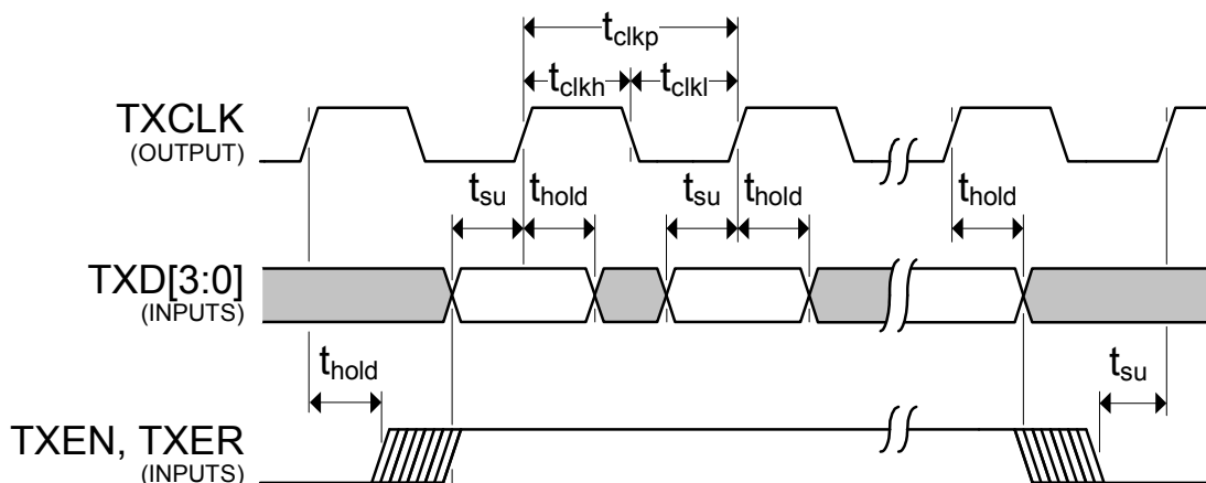
Figure 5.5 MII Transmit Timing
